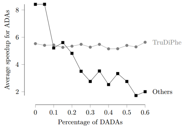
Figure 3 Average speedup of ADAs for different percentages of DADAs and a fixed amount of EGOs in ‘traditional’ systems (with reputation managers) compared to a simulation with TruDiPhe with a total of 100 agents
