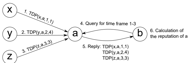
Figure 2 The schematic calculation of agent a 's reputation with TruDiPhes
